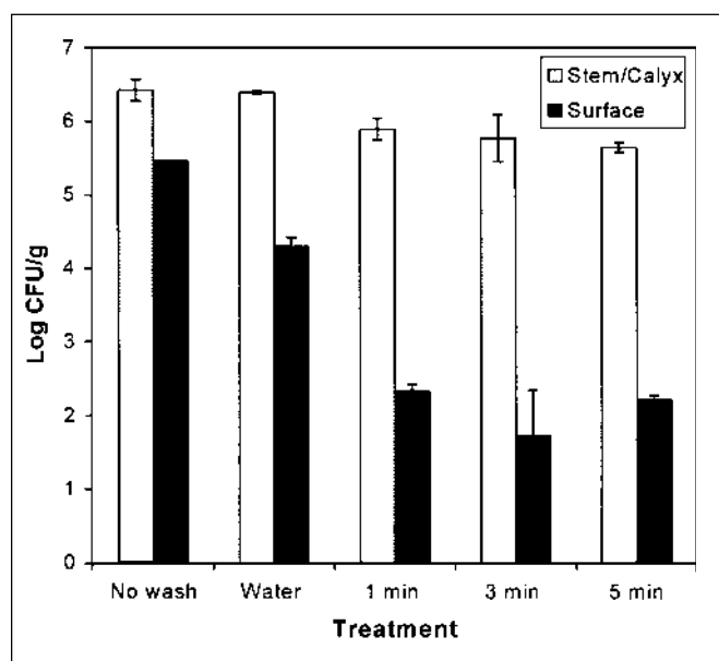
Figure 1 —Counts of Escherichia coli O157:H7 ( \log_{10} CFU/g) on inoculated apples that were unwashed, water-washed, or treated with bubbling ozone in water at 22 to 25 °C; residual ozone concentration at 1 min: 20.8 mg/L, 3min: 24.5 mg/L, and 5 min: 27.7 mg/L. Error bars represent the standard deviation of the mean of 6 apples.
